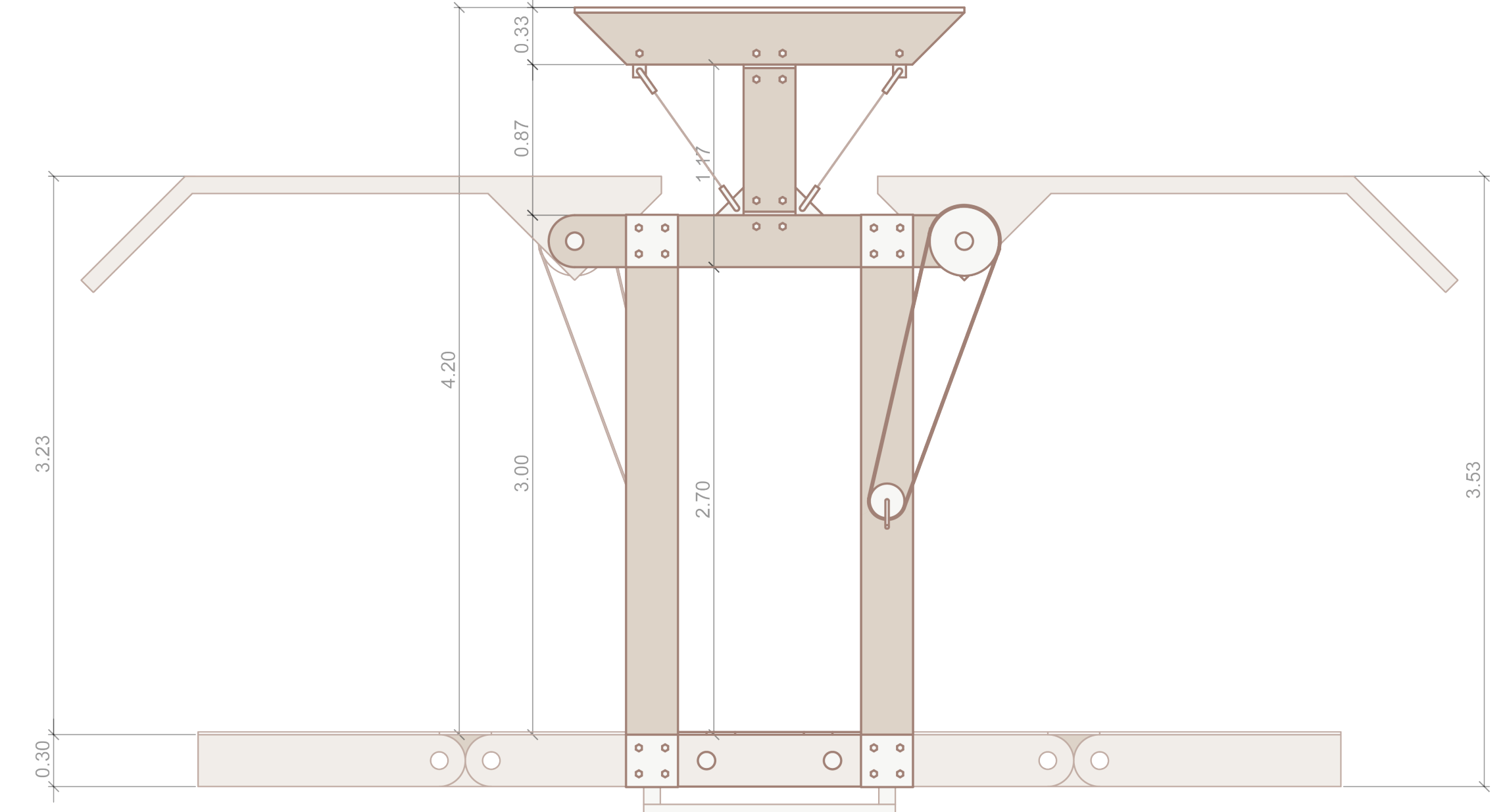
VISTA FRONTAL
