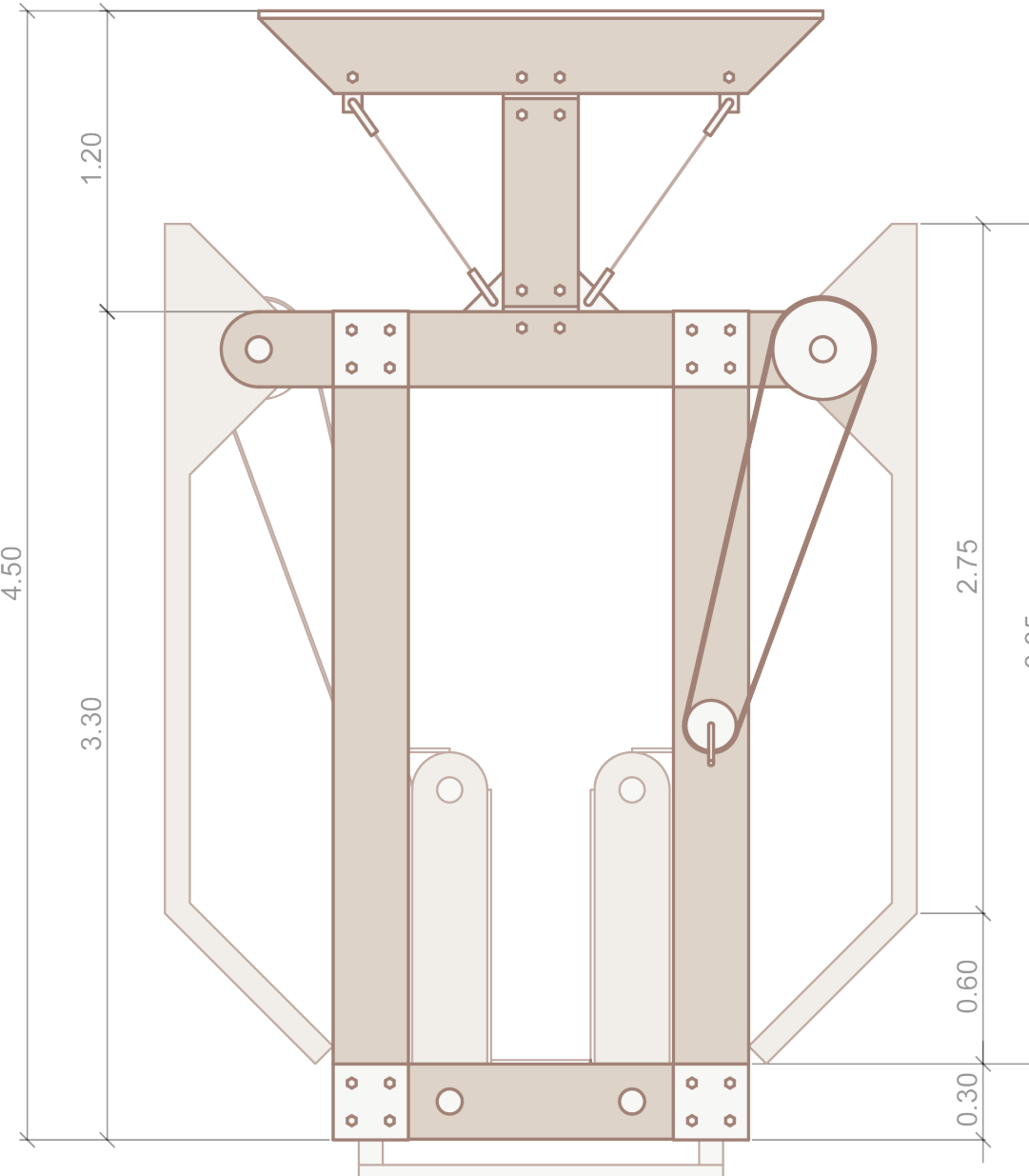
VISTA FRONTAL
