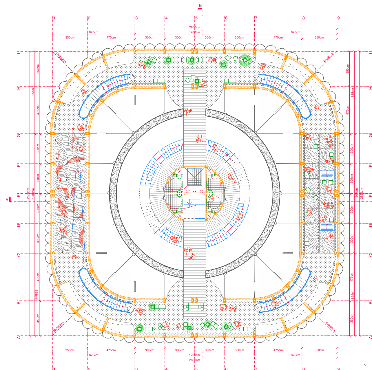
PLANTA PLAYGROUND ESCALA 1:200
