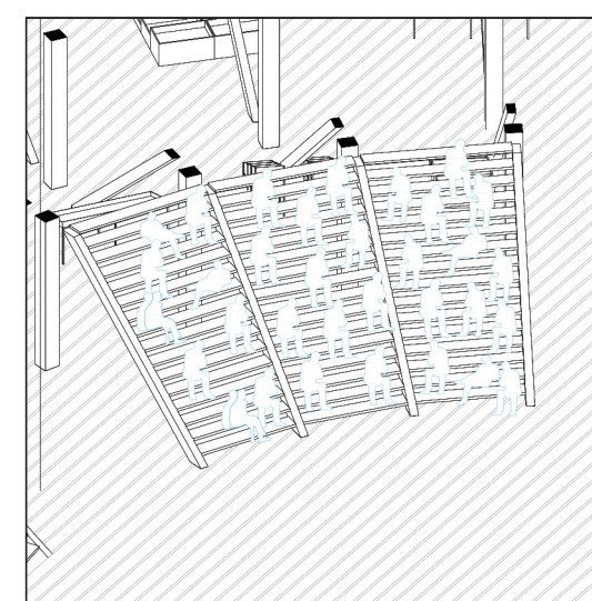
DETALLE 07 GRADERIA
