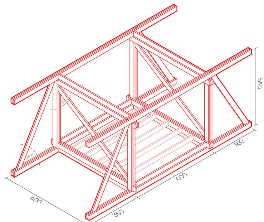
MÓDULO REPLICABLE
